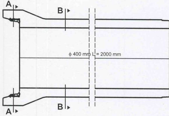
DN 400 mm ENT.CONT.BETON BORU
